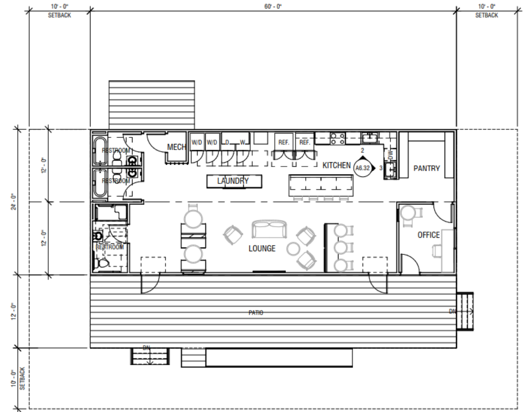
1 COMMUNITY CENTER TYPE 2 FLOOR PLAN 1/8" = 1'-0"
