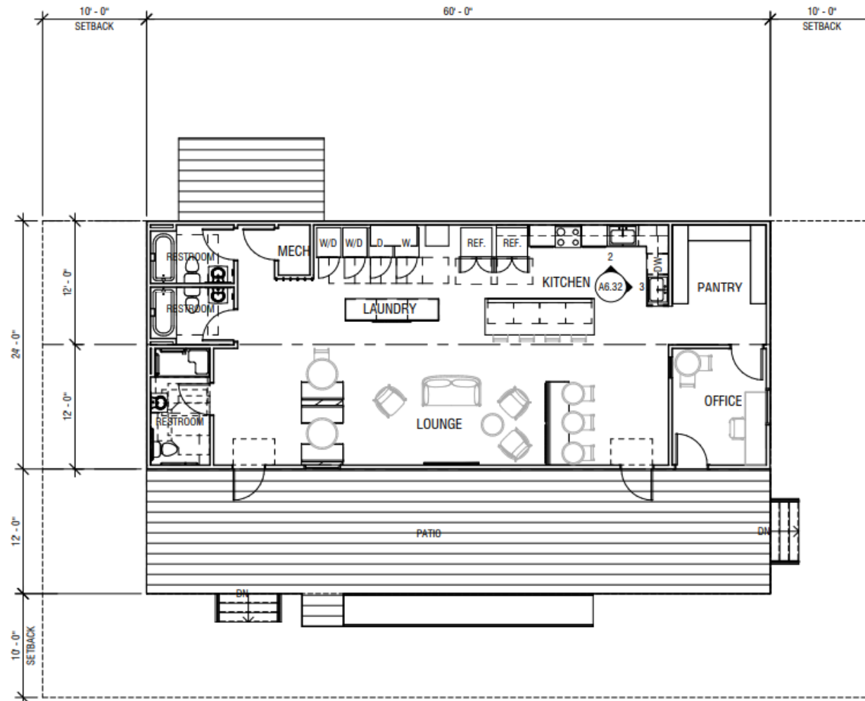
1 COMMUNITY CENTER TYPE 2 FLOOR PLAN
