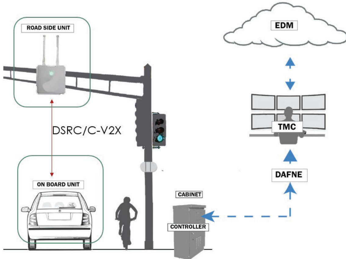
Figure 1: Connected Vehicle Systems Scope
