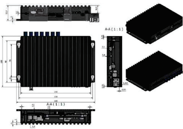
Commsignia ITS-0B4
