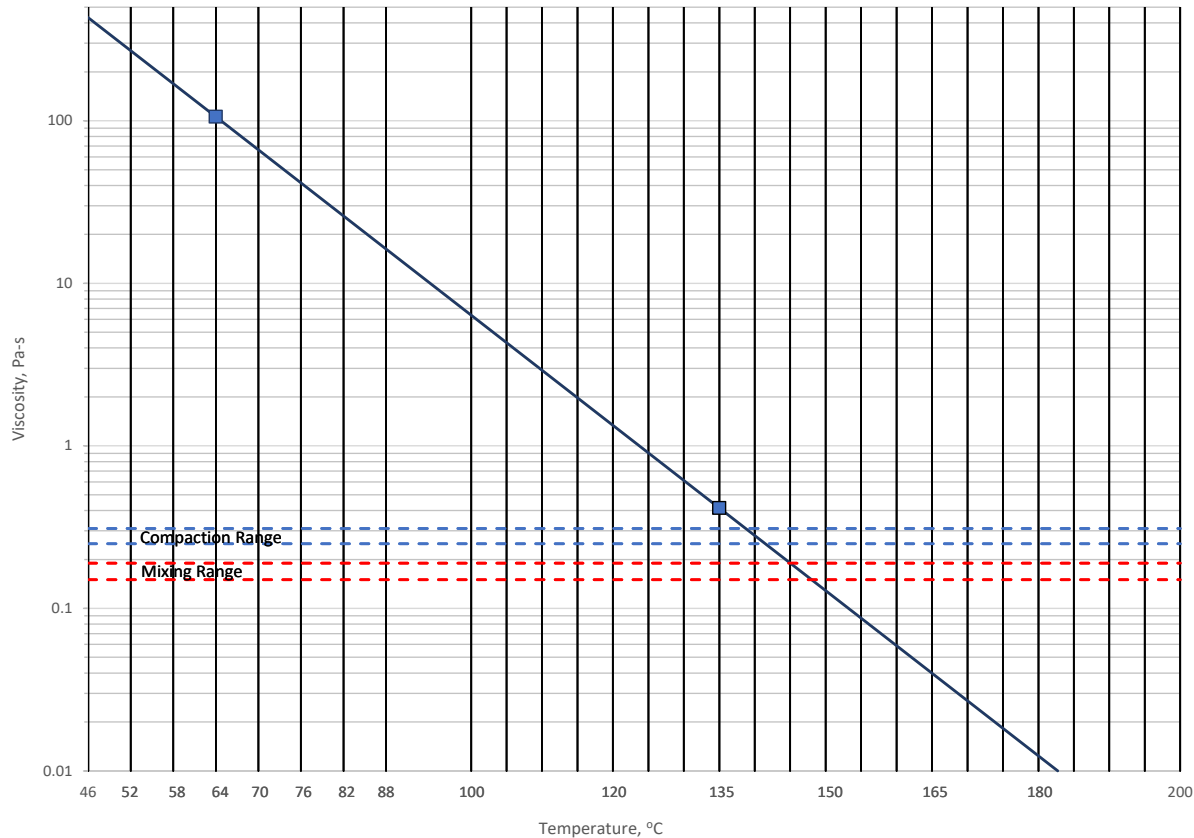
Temperature Viscosity Curve PG 64-22(25) (Product Code 101140)
