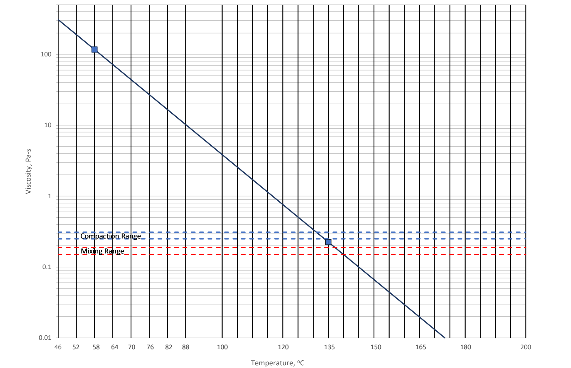
Temperature Viscosity Curve PG 58-28
