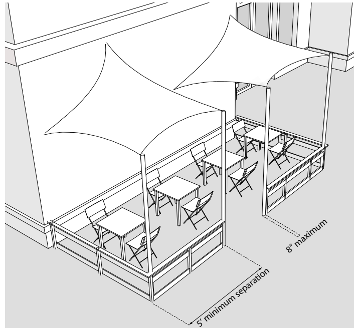
Figure 11.10-4 Delineating Elements
