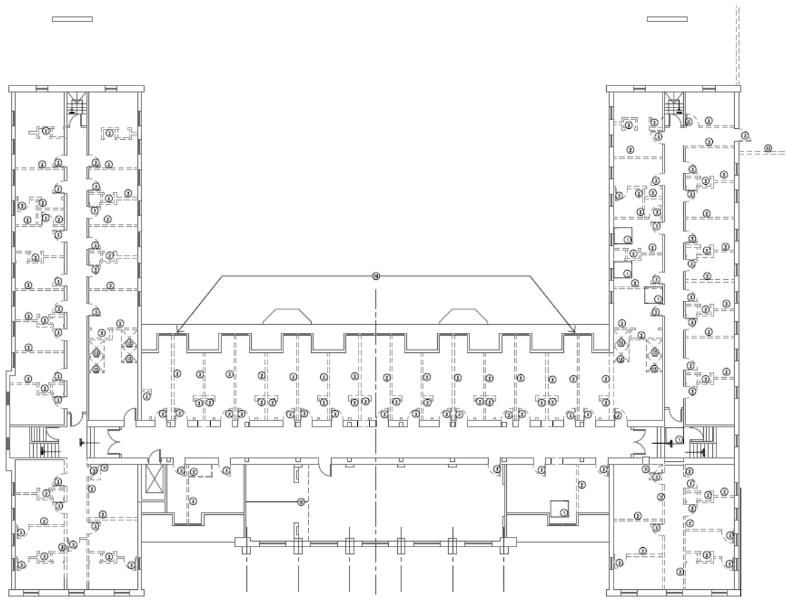
1 FOURTH FLOOR EXISTING/DEMOLITION PLAN SCALE 1/8" = 1'-0"
