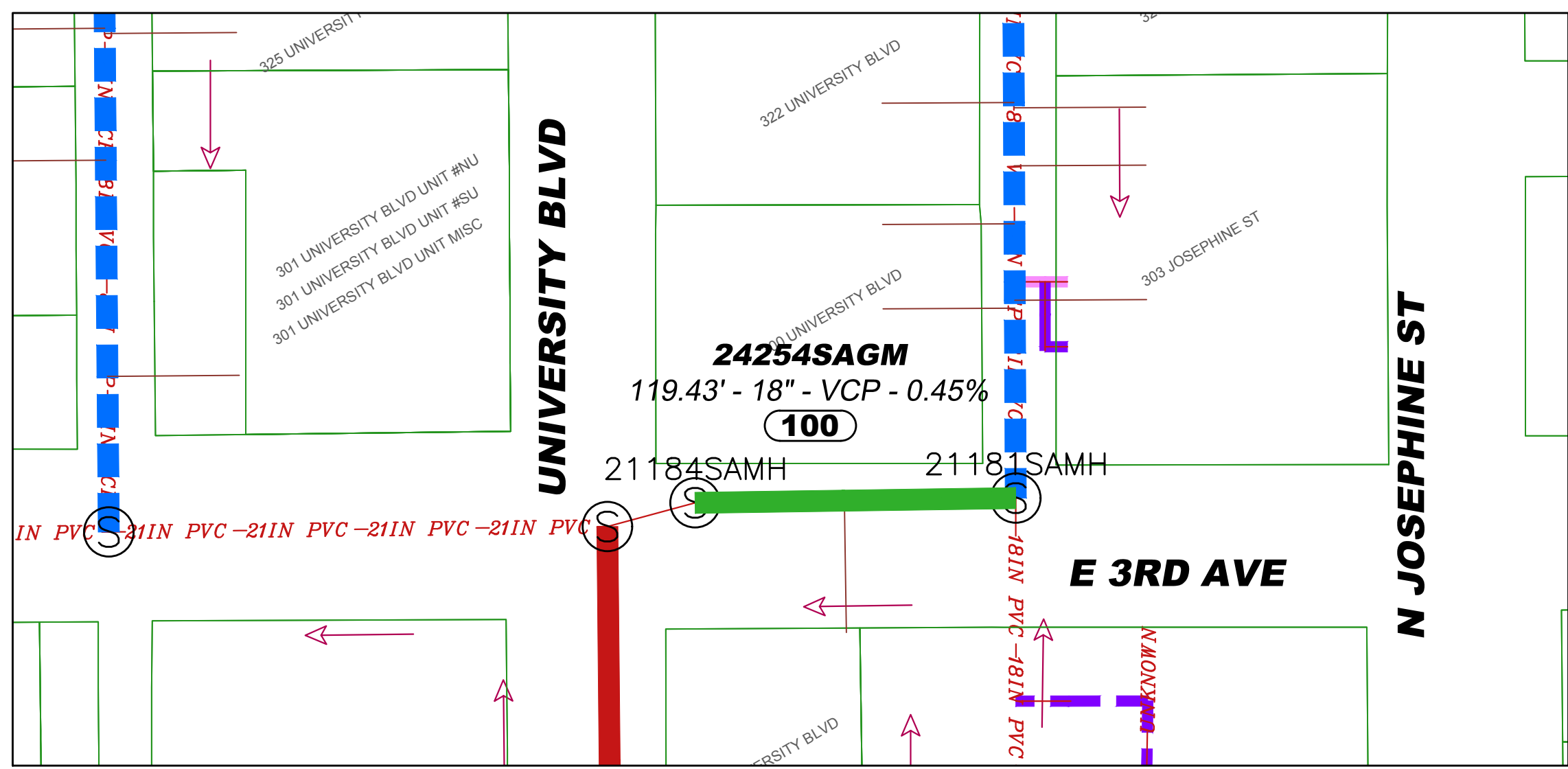
E 3RD AVE SANITARY - UNIVERSITY BLVD TO N JOSEPHINE ST
