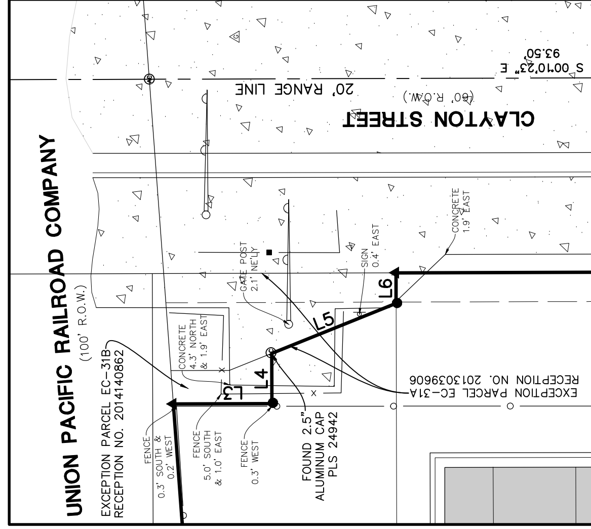
DETAIL "A" 1" = 10'
