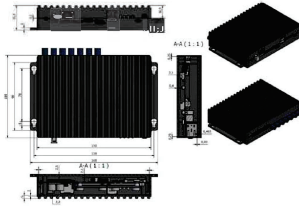
Commsignia ITS-0B4
