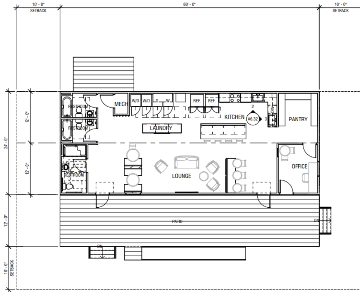
1 COMMUNITY CENTER TYPE 2 FLOOR PLAN 1/8" = 1'-0"
